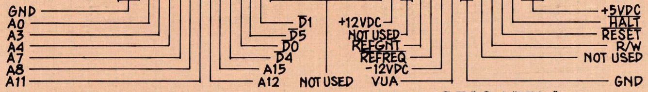
REAR VIEW
